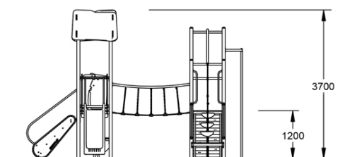
SIDE ELEVATION
